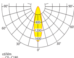
207967-SC: 6W LED-bar
