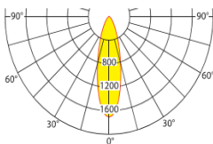
107970: 10W LED-bar
