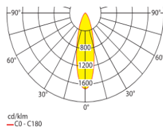
107965: 6W LED-bar
