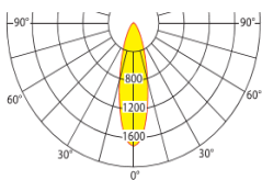
107965: 6W LED-bar
