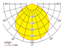
207937-SC: 6W LED-bar
