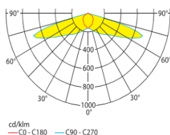
207952-SC: 6W LED-bar
