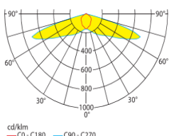
207952-SC: 6W LED-bar
